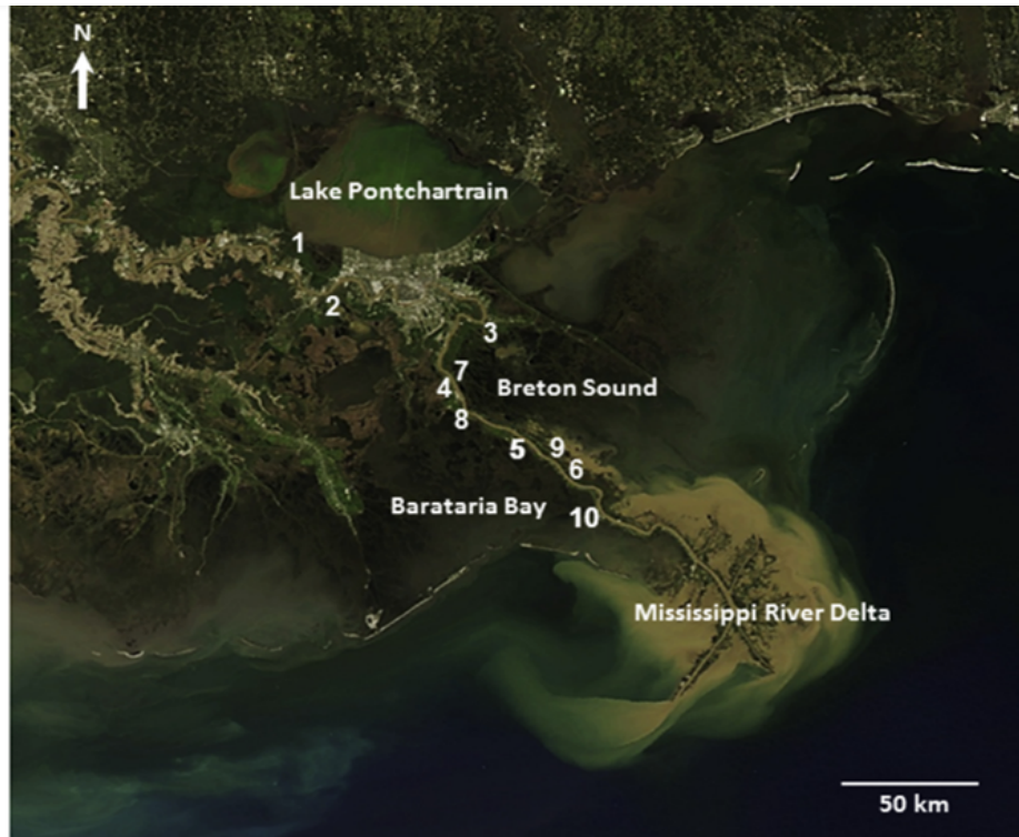
Figure 3. Existing and proposed freshwater diversions in the study area (CPRA 2017); 1– Bonnet Carré Spillway; 2– Davis Pond Diversion; 3– Caernarvon Diversion; 4- Naomi Siphon; 5– West Pointe a la Hache Siphon; 6– Bohemia Spillway; 7– Mid-Breton Sound (proposed); 8– Mid-Barataria (proposed); 9– Lower Breton Sound (proposed); 10- Lower Barataria (proposed). (Figure 2 from Bargu et. al 2019).
