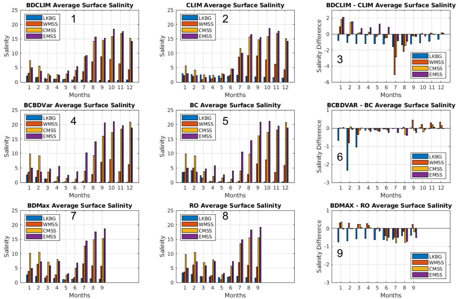
Figure 17. Monthly averages of surface salinity and differences (across twin experiments) in monthly averages of surface salinity for ROIs defined in figure 14-2. For the plots in the third column, the scenario without the Mid-Breton Diversion discharge is subtracted from the scenario containing the Mid-Breton Diversion discharge (Table 1) resulting in: Climatology Difference (BDCLIM-CLIM, panel 3), BCBDVAR Difference (BCBDVAR-BC, panel 6) and BDMAX Difference (BDMAX-RO, panel 9). Negative values in column three indicate fresher conditions associated with active MBrSD. Abbreviations are as follows: LKBG=Lake Borgne, WMSS=Western Mississippi Sound, CMSS=Central Mississippi Sound, EMSS=Eastern Mississippi Sound.
