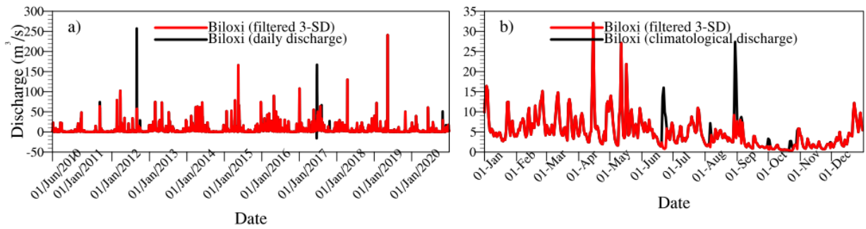
Figure A15: Interannual daily river discharge data for the Biloxi River (Station 02481000) (a) and the corresponding daily climatological discharge (b).
