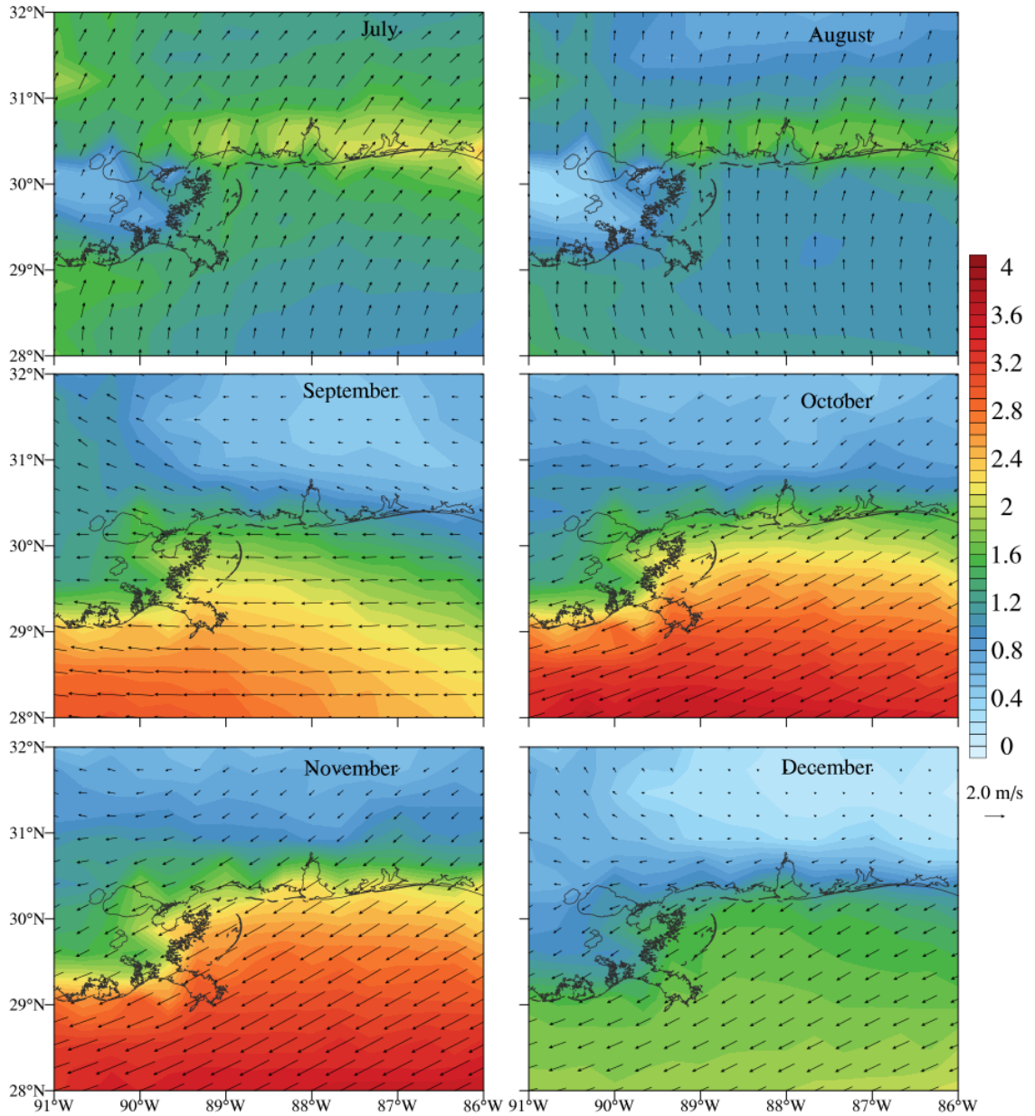
Figure 11. Spatial pattern of climatological (2010-2020) monthly mean wind distribution over the study region estimated from NARR. The Wind speed (m/s) is indicated by the colored field and the scaled wind vectors reveal both wind direction and magnitude for July to December. The spatial resolution of the NARR wind field is 32 km, which is represented by the spacing of the wind vectors.
